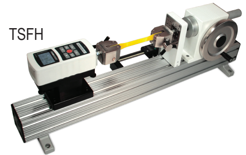
The TSFH is shown in a tensile test, with Series 5 digital force gauge, film and paper grips, and digital travel display
